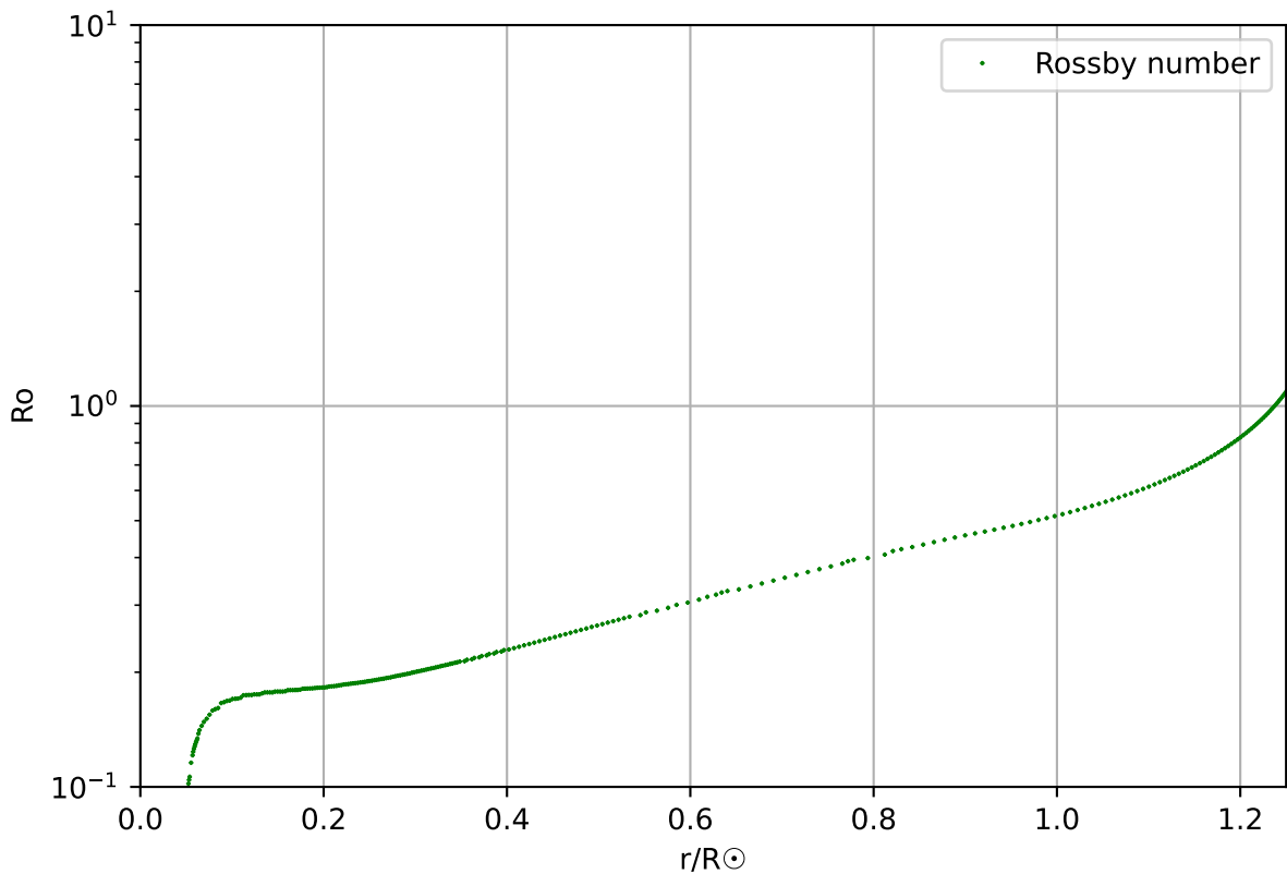
Rossby number, profile 172, age 10.0 \times 10^9
